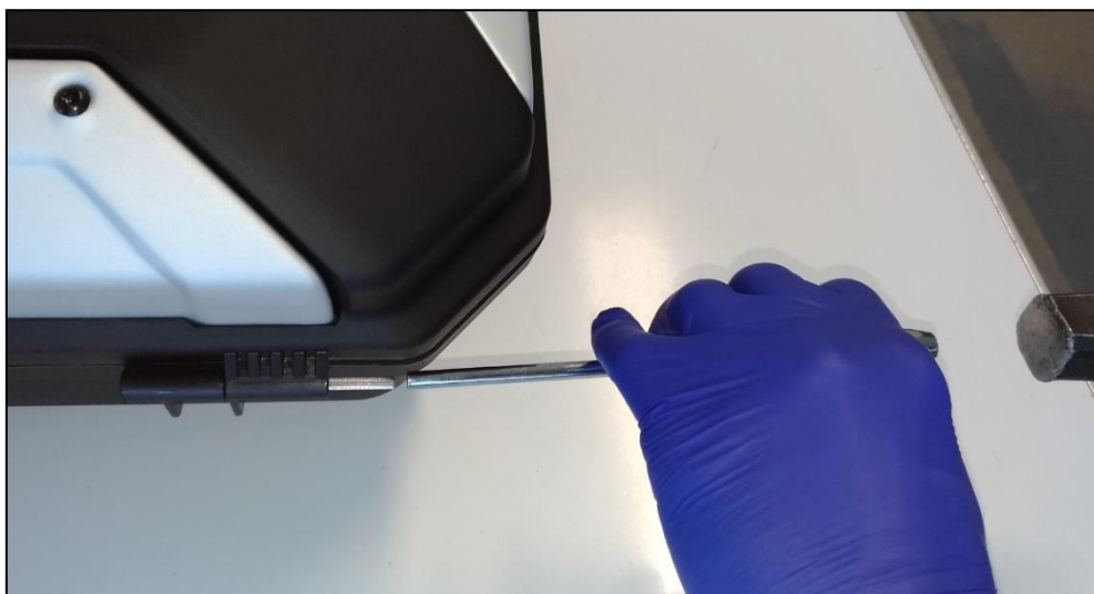
Photo 3: use of the pin punch to insert the pin into the hinges
